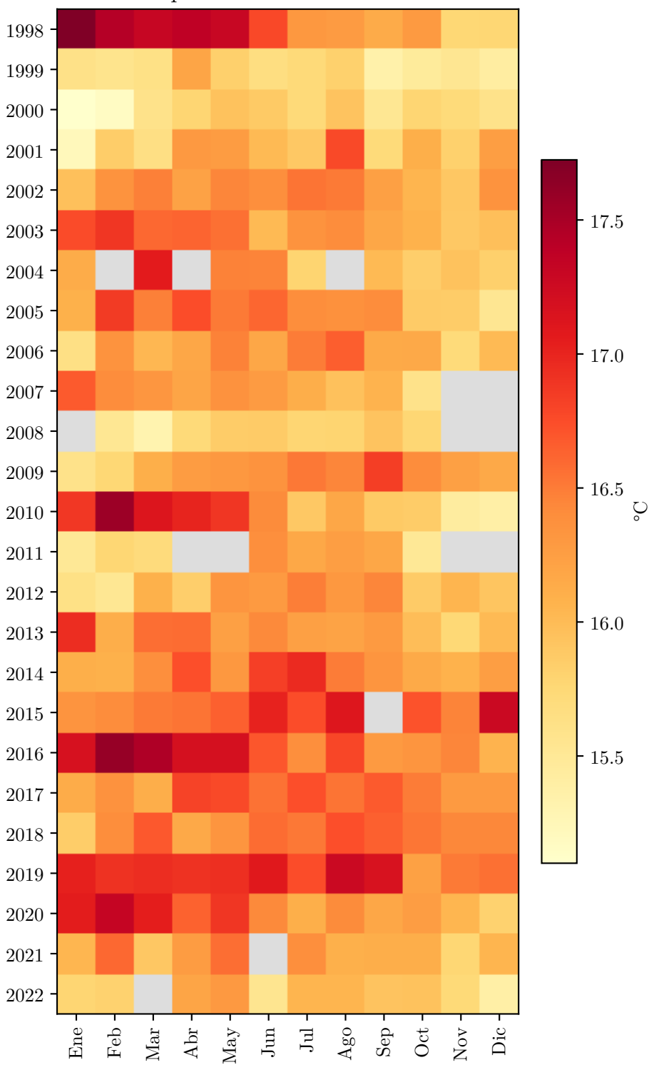
Temperatura media ERA5-Land
